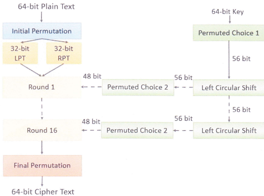
Data Encryption Standard (DES)
