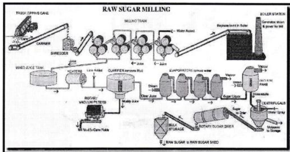
Figure 2.1 Schematic view of sugar production
