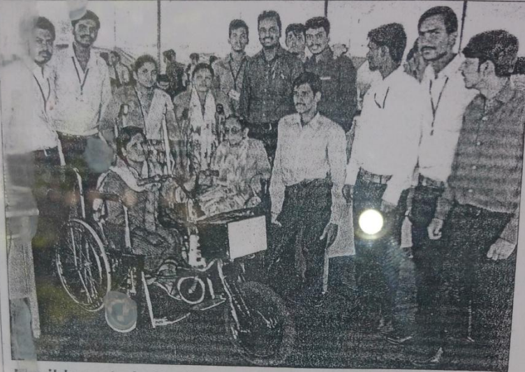
Flexible seated wheel chair for physically challenged and economically poor developed by students of HiraSugar Institute of Technology, Nidasoshi. DH PHOTO
