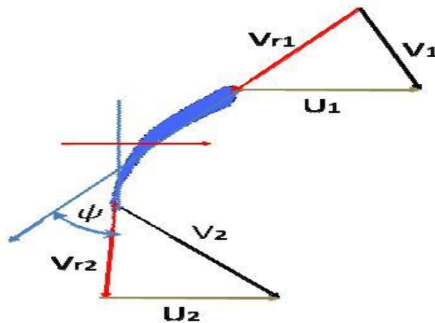
Fig. 1 Flow across a compressor blade
