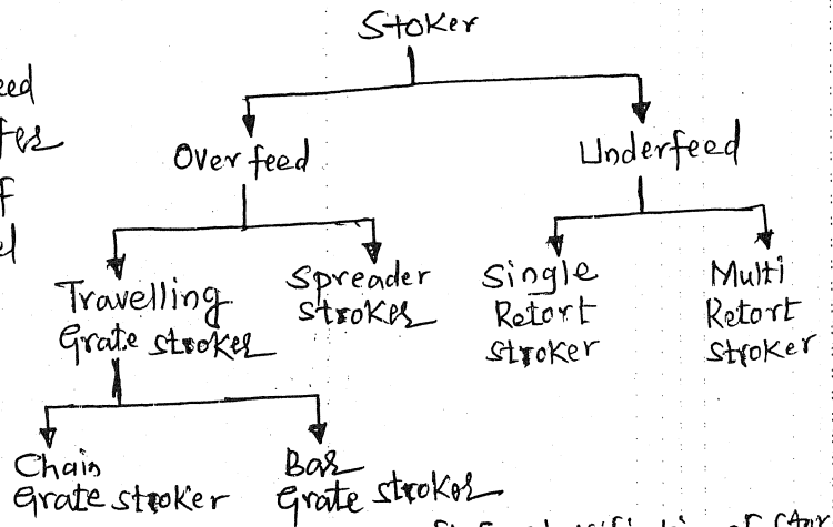
fig 5. Classification of stokers
